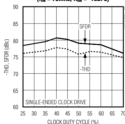
-THD, SFDR vs. CLOCK DUTY CYCLE ( f_{IN} = 70MHz , A_{IN} = -1dBFS )
